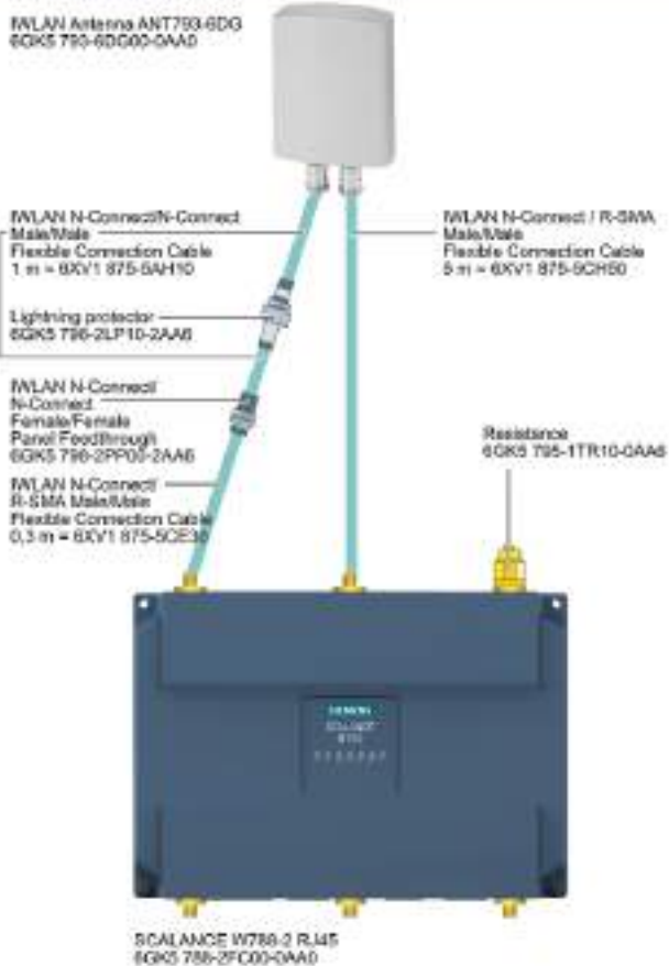
Dual Beam antenna ANT793-6DG connected to SCALANCE W788-2 RJ45 with R-SMA ports
